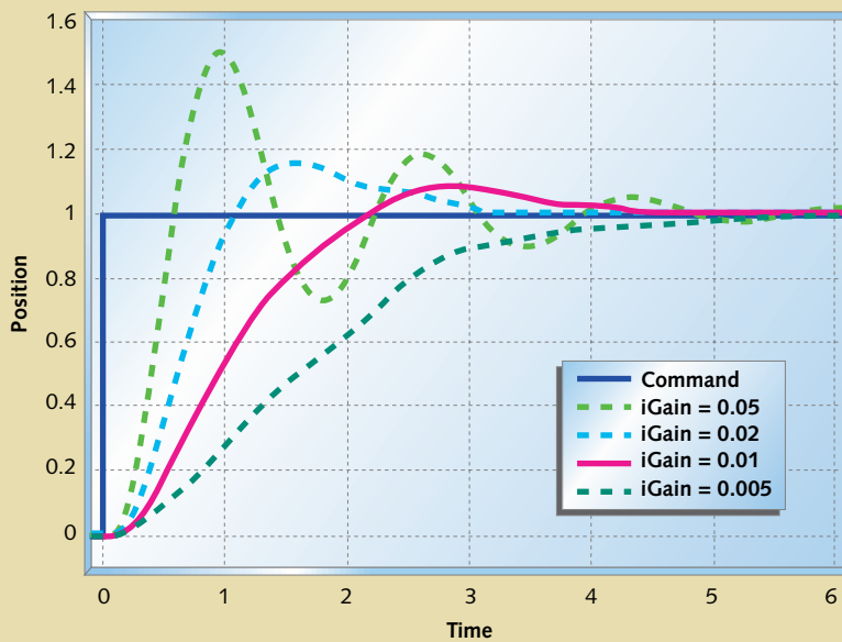
FIGURE 12 Temperature control system with integral control. The kink at time = 2 is from the external disturbance
