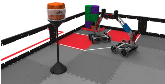
Figure 19: Example of a Robot contacting an opponent Robot that is fully contained within its Protected Zone.
